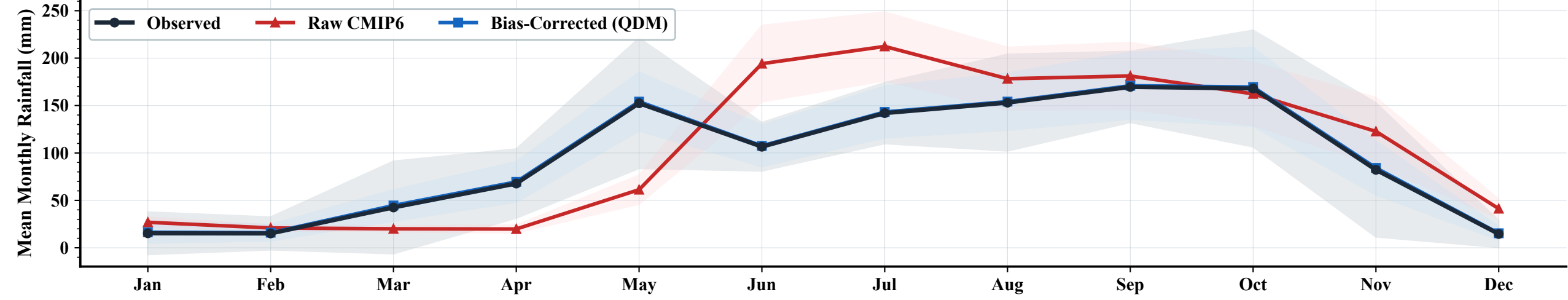
Regional Mean Monthly Climatology (1- shading)
